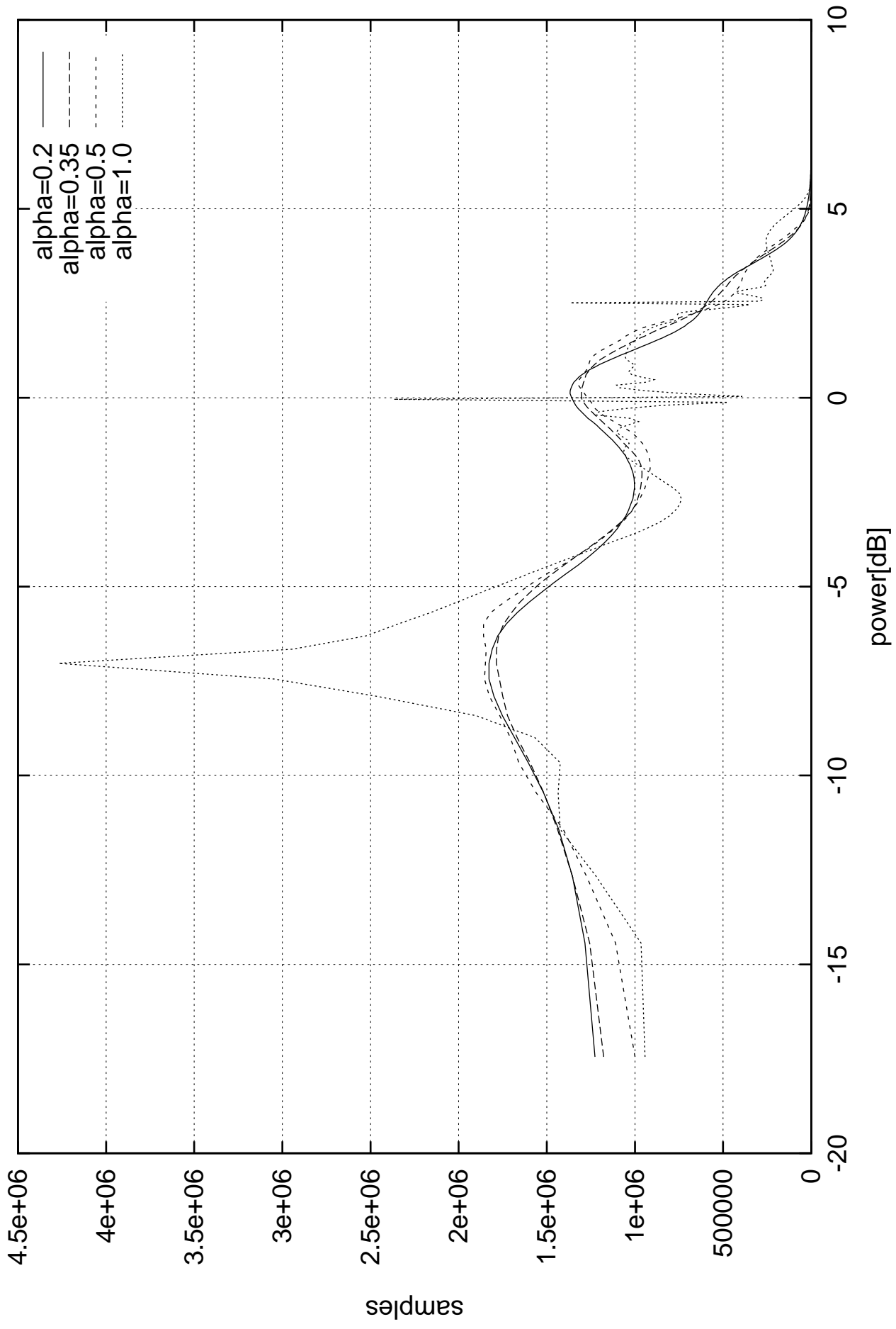
16QAM power histogram (PN23, root rolloff)
